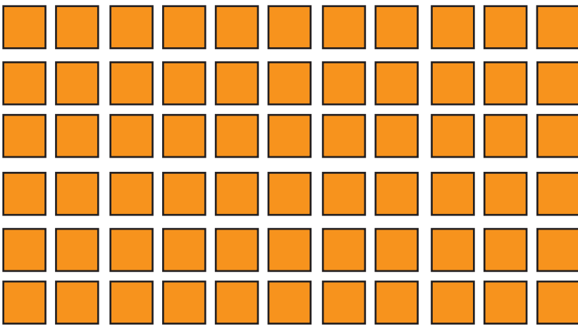
Squares
